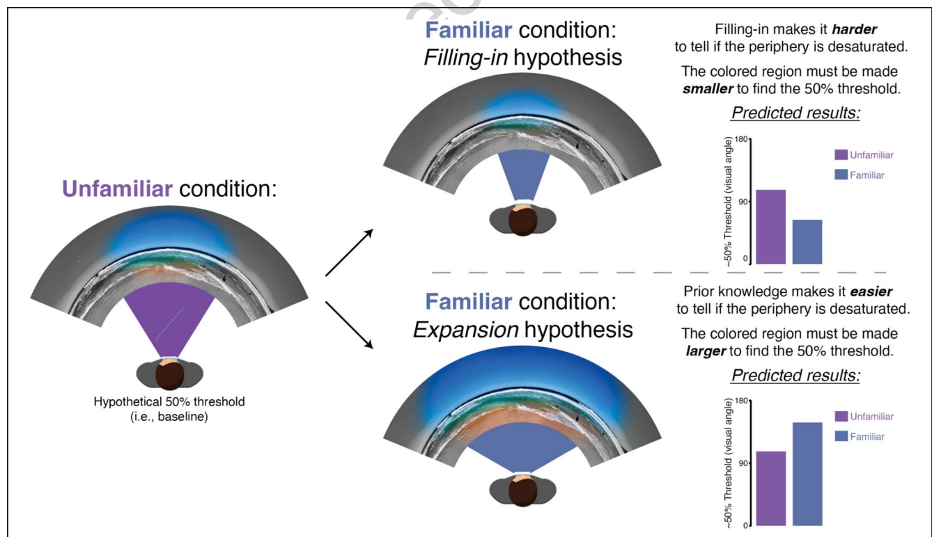
Figure 4. Potential experimental outcomes with the current design. The left image represents the hypothetical ~50% threshold when participants are unfamiliar with the stimuli. This can be thought of as the baseline condition. The top right image represents the prediction made by the filling-in hypothesis. The bottom right image represents the prediction made by the expansion hypothesis.
