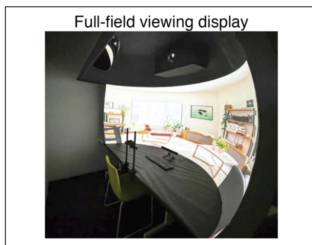
Figure 1. Picture of the full field viewing display used in both experiments. Note the chin rest, the eye-tracker, and how the display wraps around to the ends of the table (i.e., 180° of visual angle).
