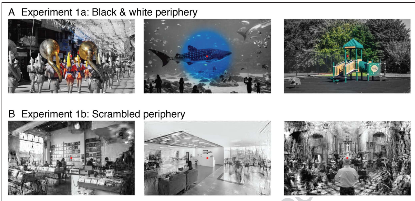
Figure 2. Sample stimuli and results from Experiments 1a (A) and 1b (B). For each experiment, example stimuli are shown during the thresholding process (although note that when presented in the experiment, they were presented on curved displays that took up of the participants' entire visual field along the horizontal axis).
