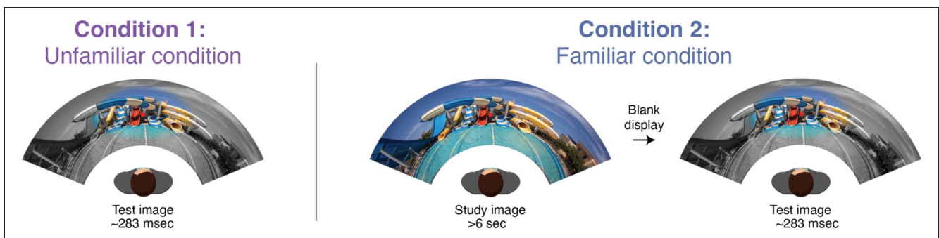
Figure 3. Visualization of one trial for the two experimental conditions. Left image: unfamiliar condition in which participants are shown the test image for approximately 283 msec. Right image: familiar condition in which participants are shown a study image that has not been altered for a minimum of 6 sec before being shown the altered test image for approximately 283 msec.
