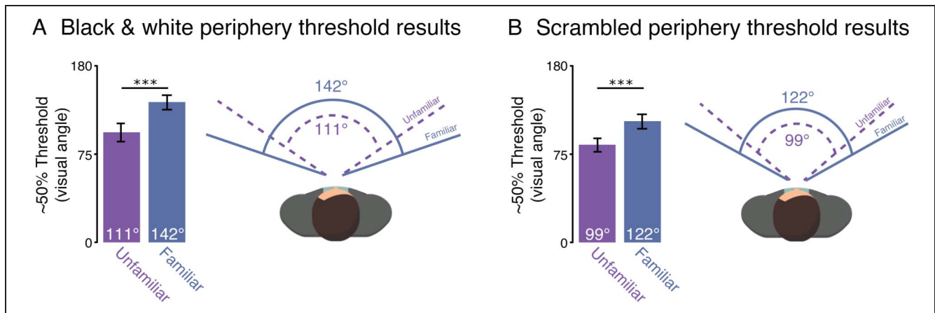
Figure 5. Experiment 1 results. (A) Experiment 1a (black and white periphery). (B) Experiment 1b (scrambled periphery). The y axis represents the output of the QUEST procedure in identifying the \sim 50\% threshold at which participants were at chance in determining if the image has been altered in the periphery or not. Purple bars represent the unfamiliar condition, and blue bars represent the familiar condition. Error bars represent the standard error of the mean. In addition, diagrams visualize the size of the unfamiliar and familiar thresholds relative to an observer's field of view. *** p < .001 .
