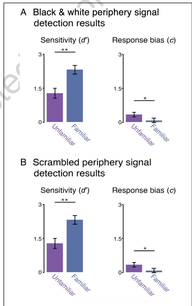
Figure 6. Experiment 2 results. (A) Experiment 2a (black and white periphery). (B) Experiment 2b (scrambled periphery). The y axis represents d' (perceptual sensitivity) or c (response bias). Purple bars represent the unfamiliar condition, and blue bars represent the familiar condition. Error bars represent the standard error of the mean. * p < .05 ; ** p < .01 .
